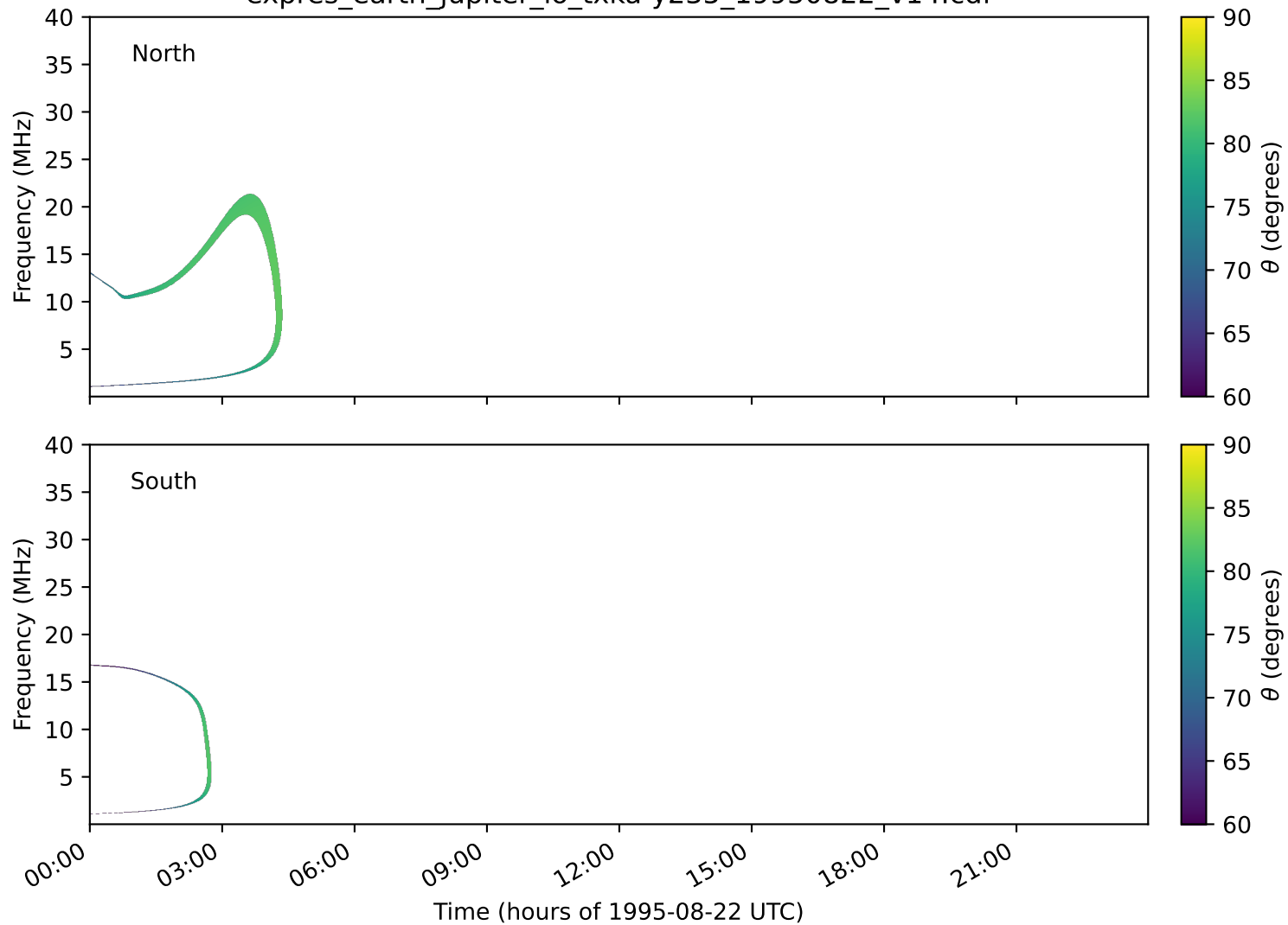
expres_earth_jupiter_io_txka-y235_19950822_v14.cdf
