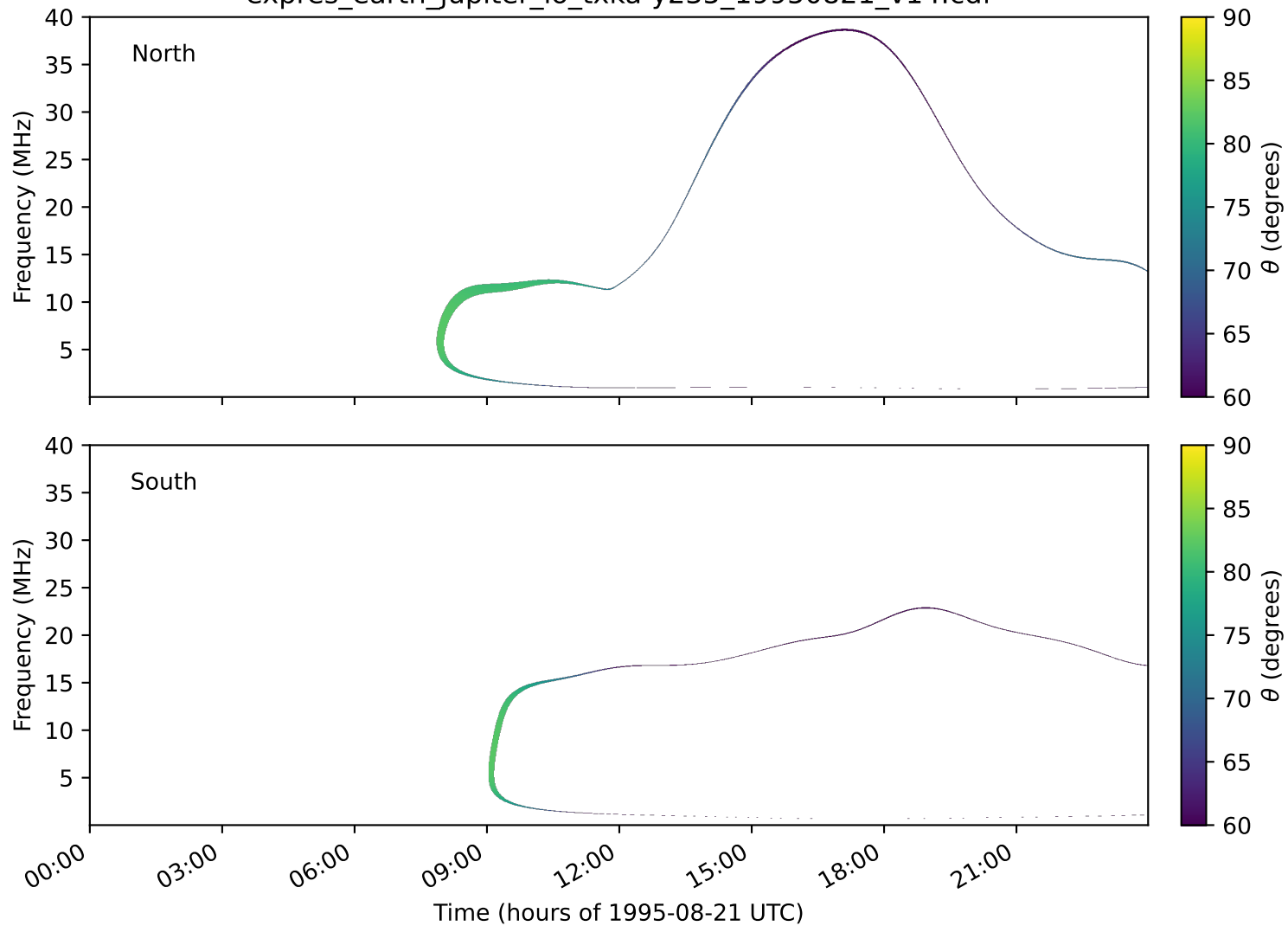
expres_earth_jupiter_io_txka-y235_19950821_v14.cdf
