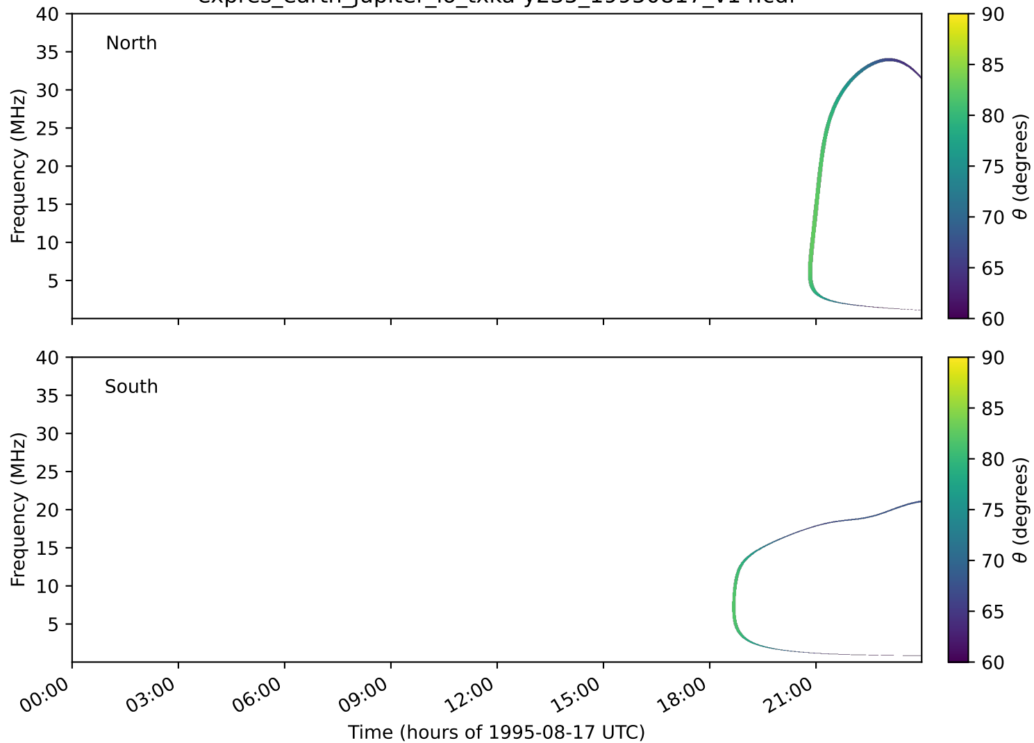
expres_earth_jupiter_io_txka-y235_19950817_v14.cdf
