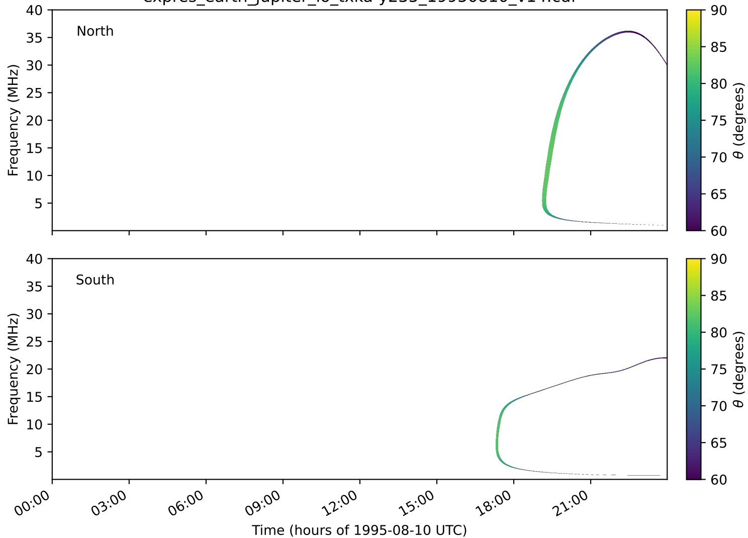
expres_earth_jupiter_io_txka-y235_19950810_v14.cdf
