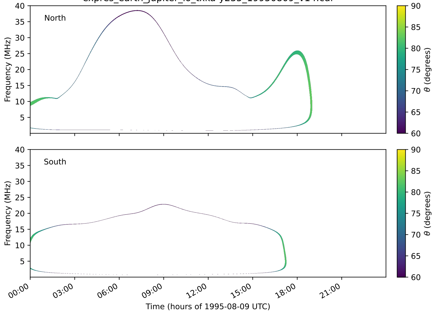
expres_earth_jupiter_io_txka-y235_19950809_v14.cdf
