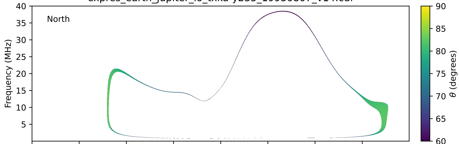
expres_earth_jupiter_io_txka-y235_19950807_v14.cdf
