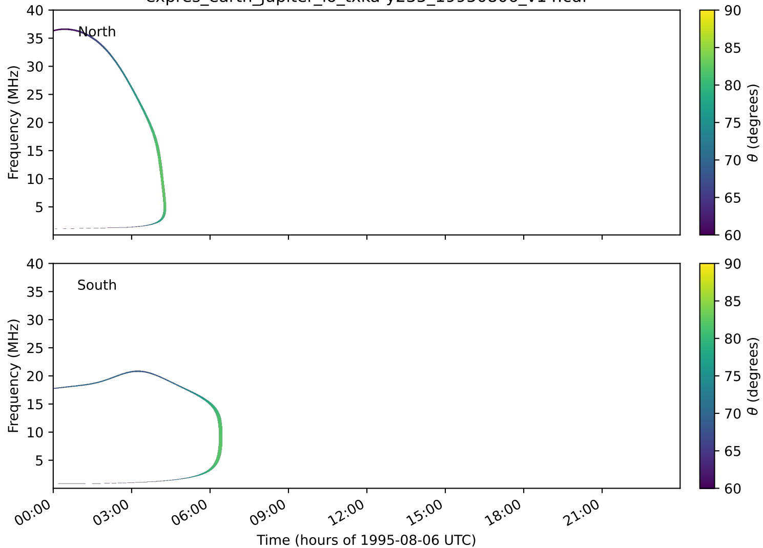
expres_earth_jupiter_io_txka-y235_19950806_v14.cdf
