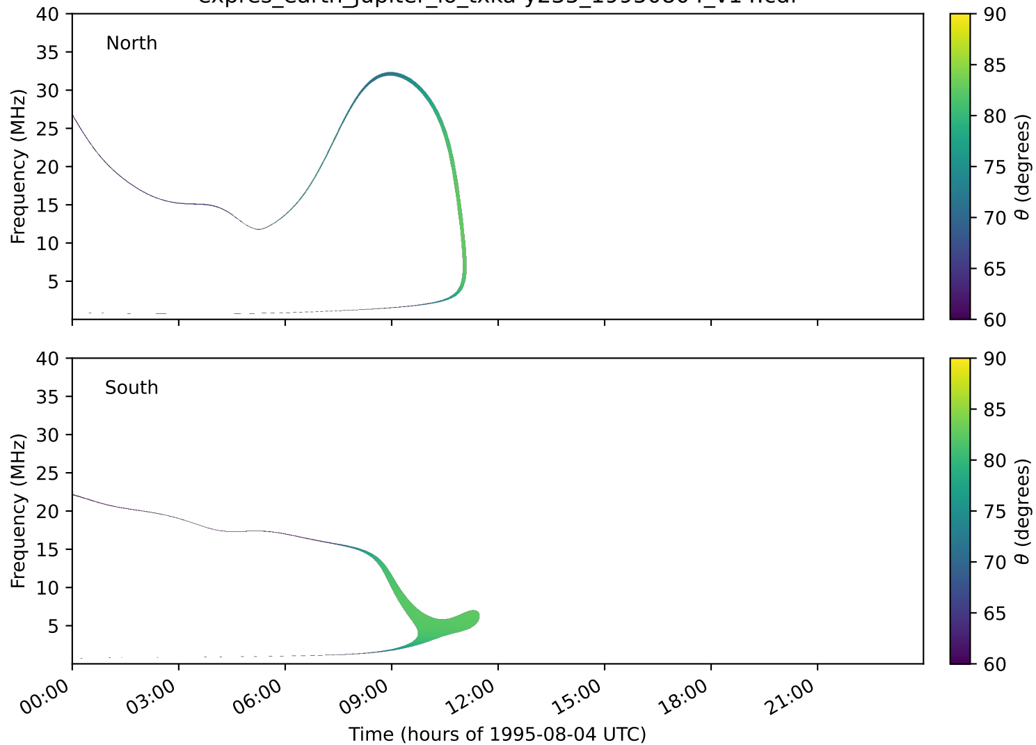
expres_earth_jupiter_io_txka-y235_19950804_v14.cdf
