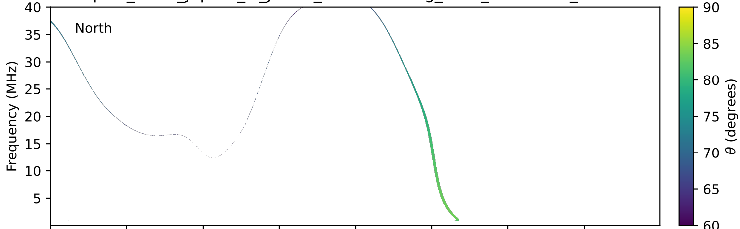
expres_earth_jupiter_io_jrm33_lossc-wid1deg_3kev_19950825_v11.cdf
