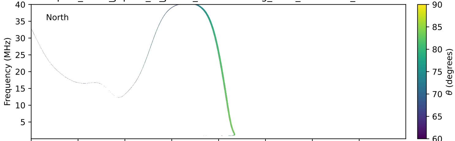
expres_earth_jupiter_io_jrm33_lossc-wid1deg_3kev_19950811_v11.cdf
