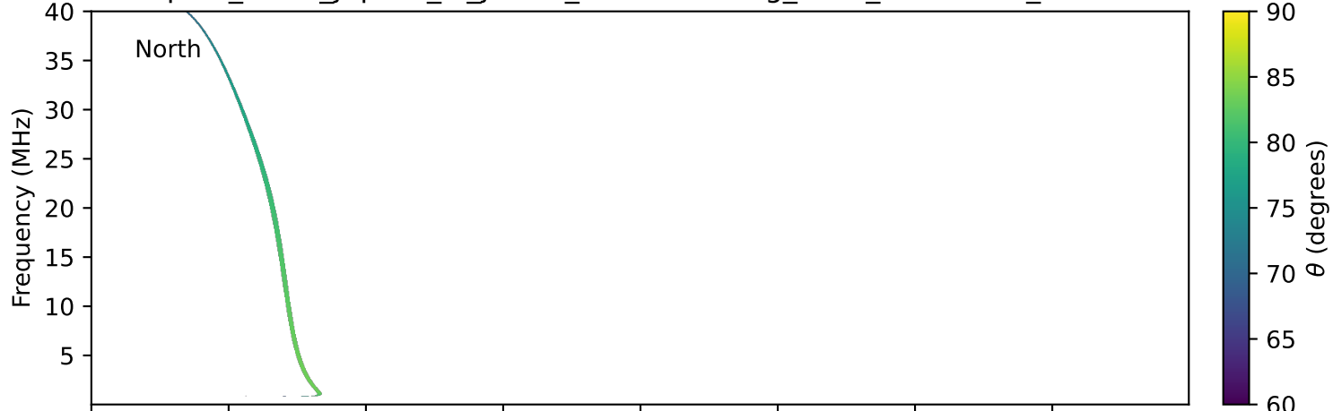
expres_earth_jupiter_io_jrm33_lossc-wid1deg_3kev_19950806_v11.cdf
