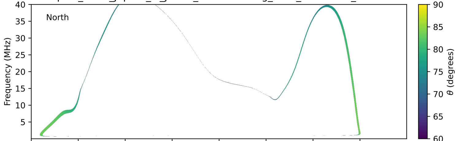
expres_earth_jupiter_io_jrm09_lossc-wid1deg_3kev_19950816_v11.cdf
