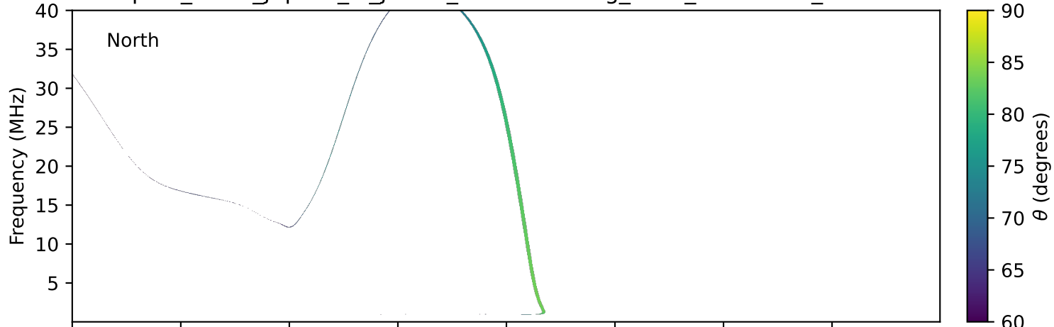
expres_earth_jupiter_io_jrm09_lossc-wid1deg_3kev_19950811_v11.cdf
