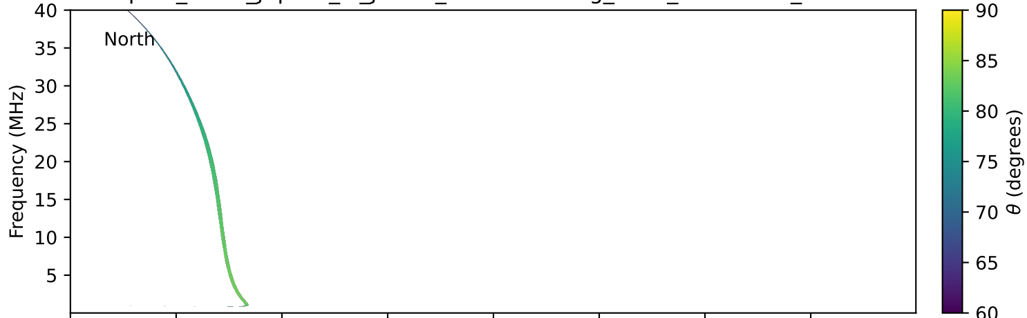
expres_earth_jupiter_io_jrm09_lossc-wid1deg_3kev_19950806_v11.cdf
