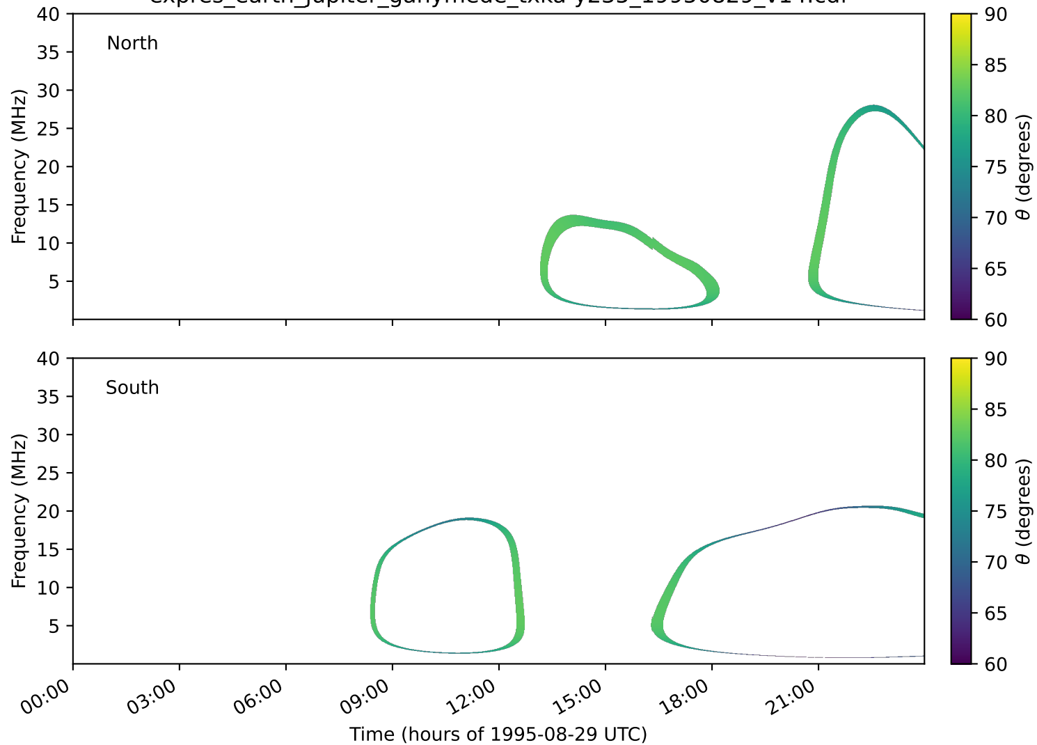
expres_earth_jupiter_ganymede_txka-y235_19950829_v14.cdf
