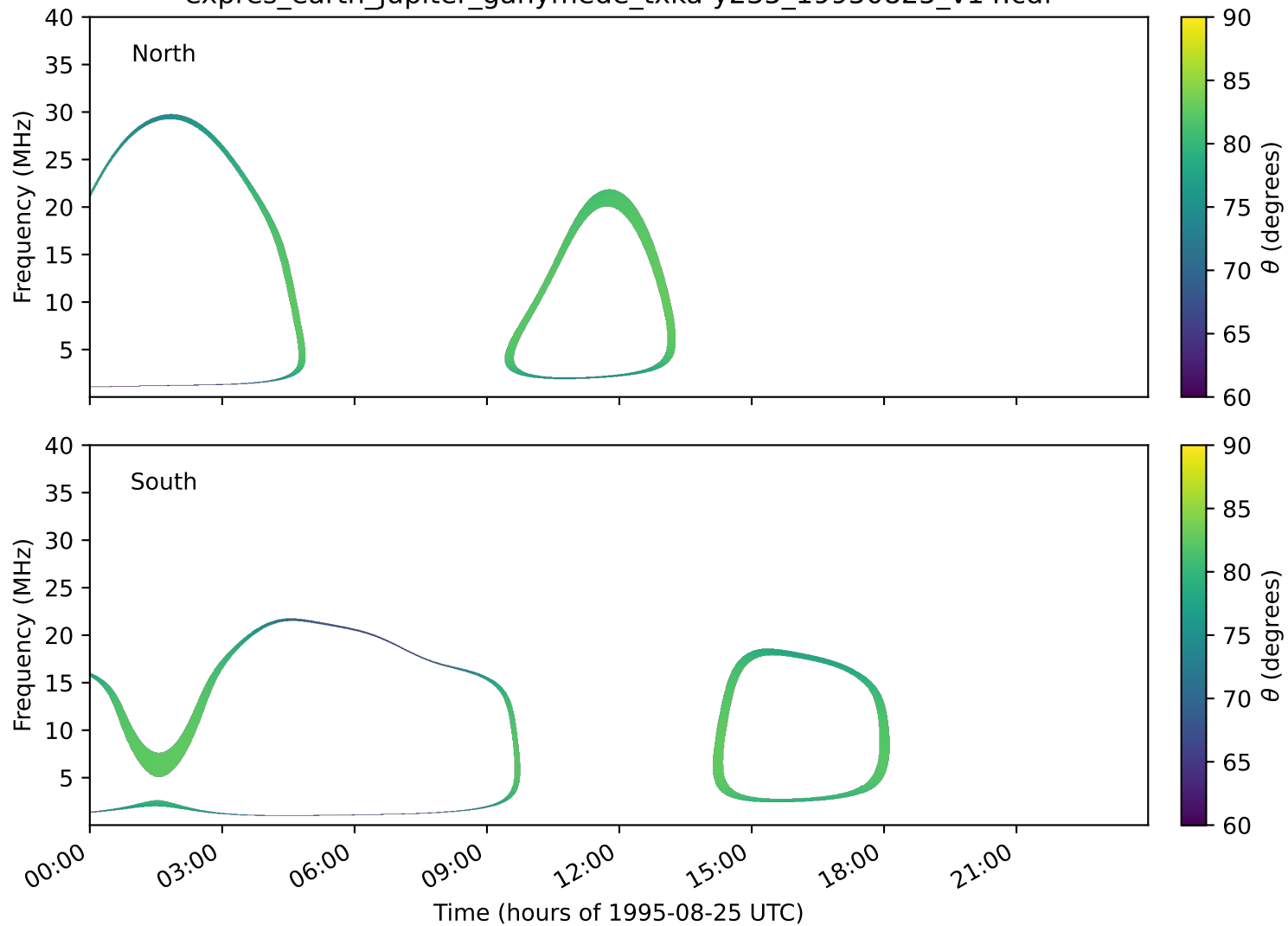
expres_earth_jupiter_ganymede_txka-y235_19950825_v14.cdf
