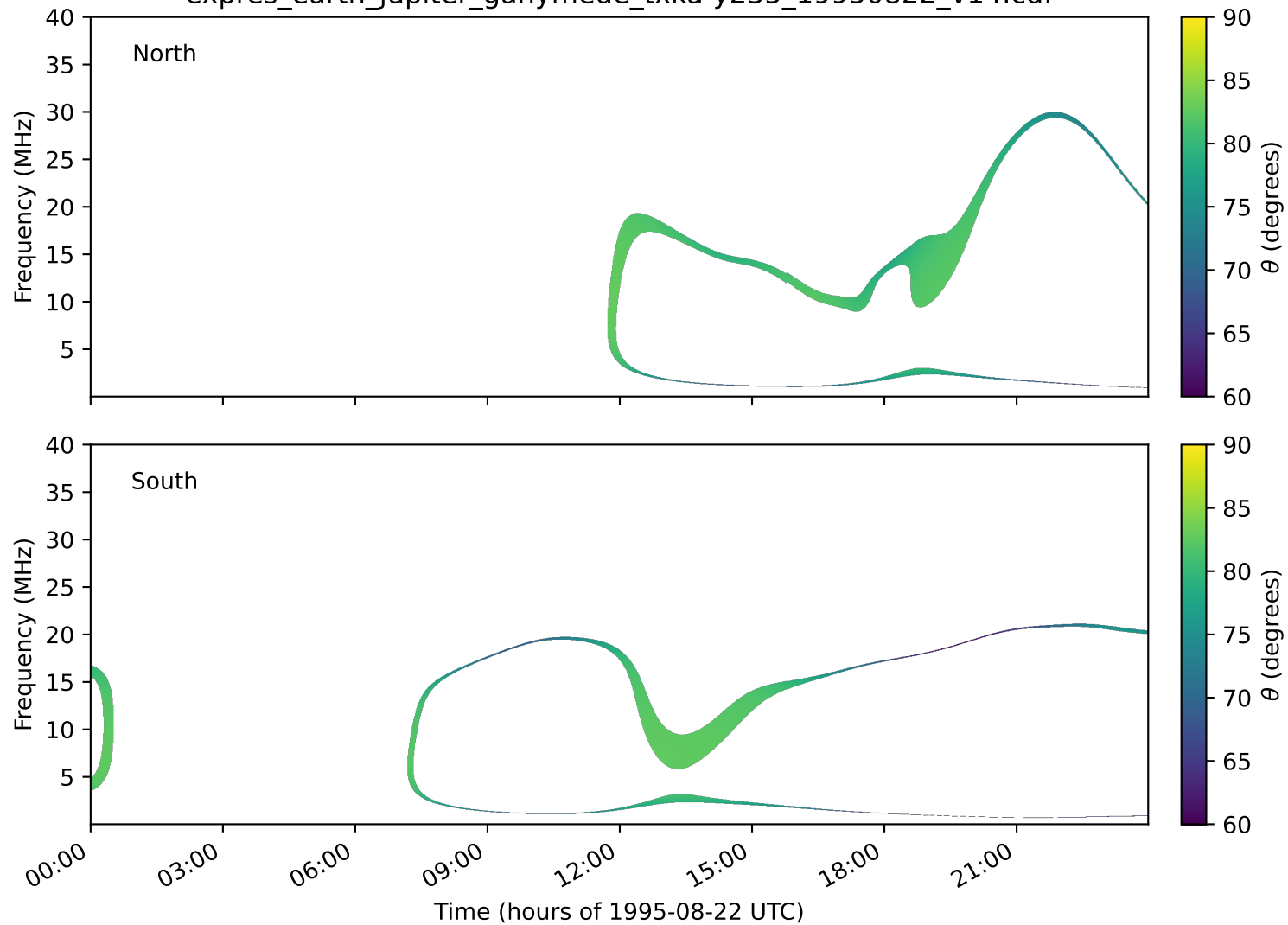
expres_earth_jupiter_ganymede_txka-y235_19950822_v14.cdf
