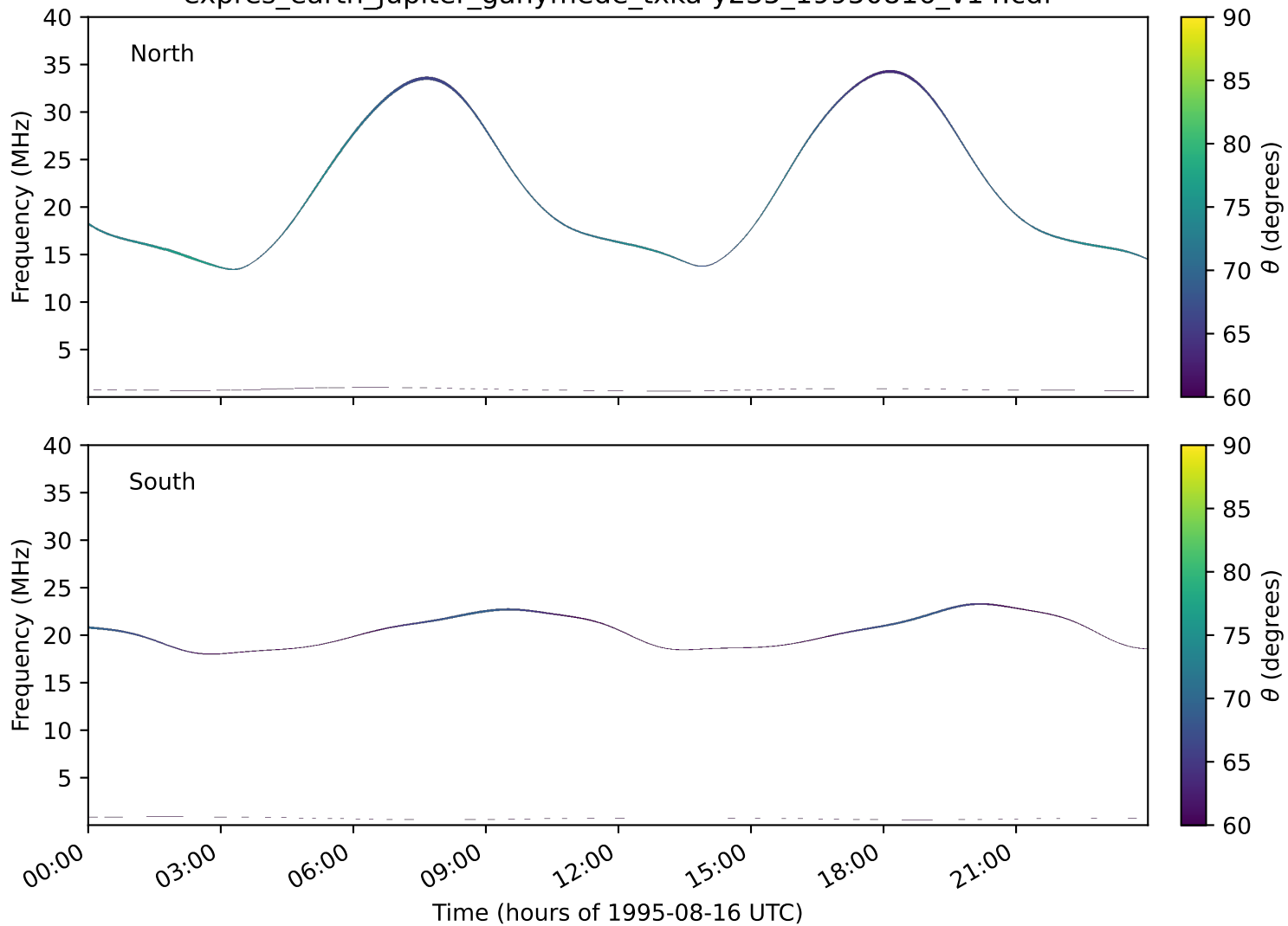
expres_earth_jupiter_ganymede_txka-y235_19950816_v14.cdf
