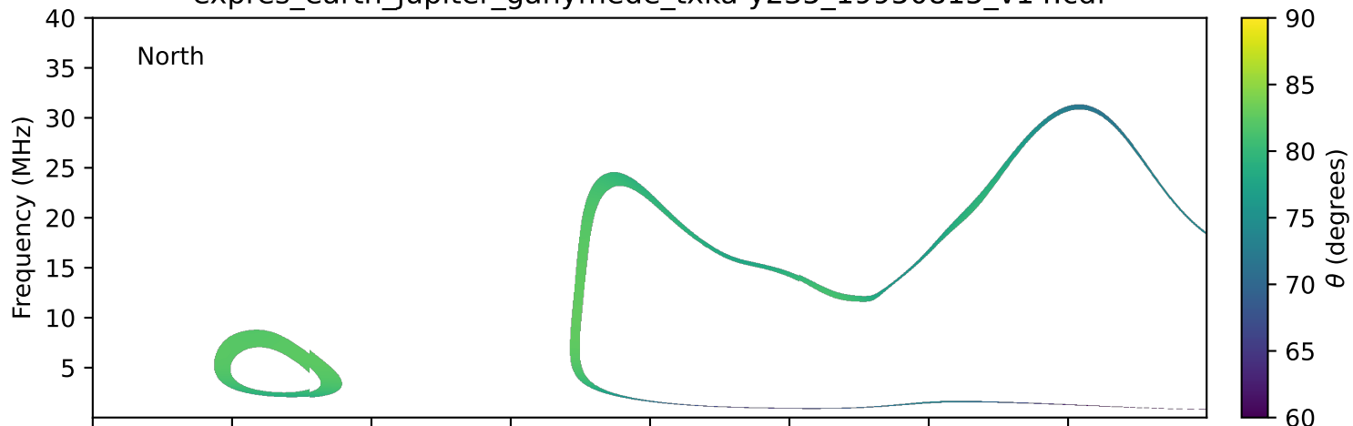
expres_earth_jupiter_ganymede_txka-y235_19950815_v14.cdf
