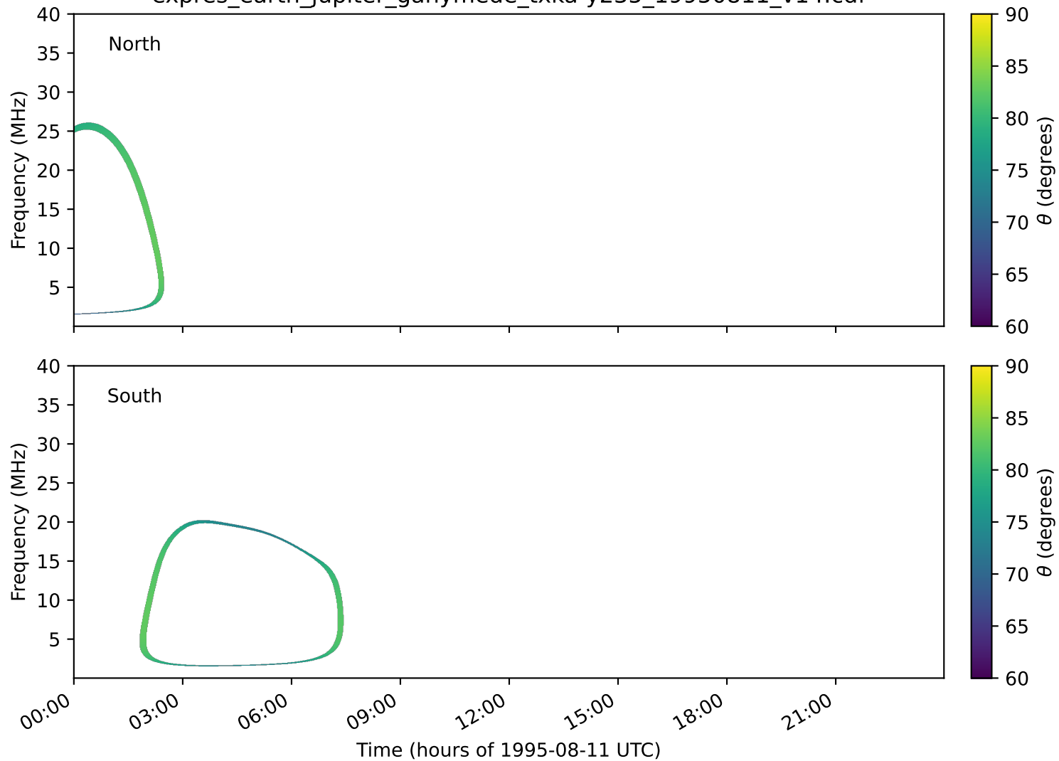
expres_earth_jupiter_ganymede_txka-y235_19950811_v14.cdf
