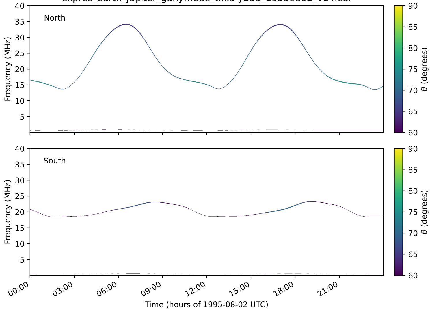
expres_earth_jupiter_ganymede_txka-y235_19950802_v14.cdf
