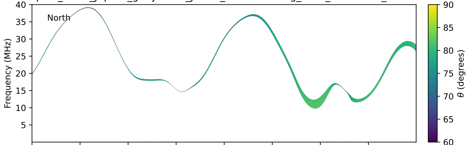
expres_earth_jupiter_ganymede_jrm33_lossc-wid1deg_3kev_19950803_v11.cdf
