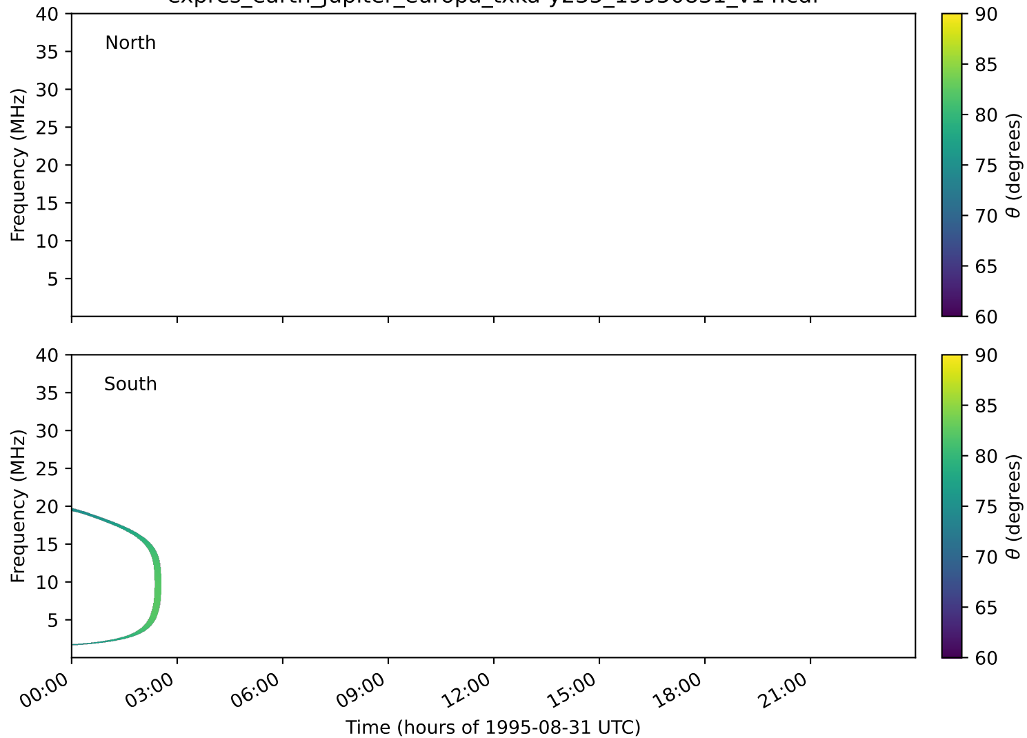
expres_earth_jupiter_europa_txka-y235_19950831_v14.cdf
