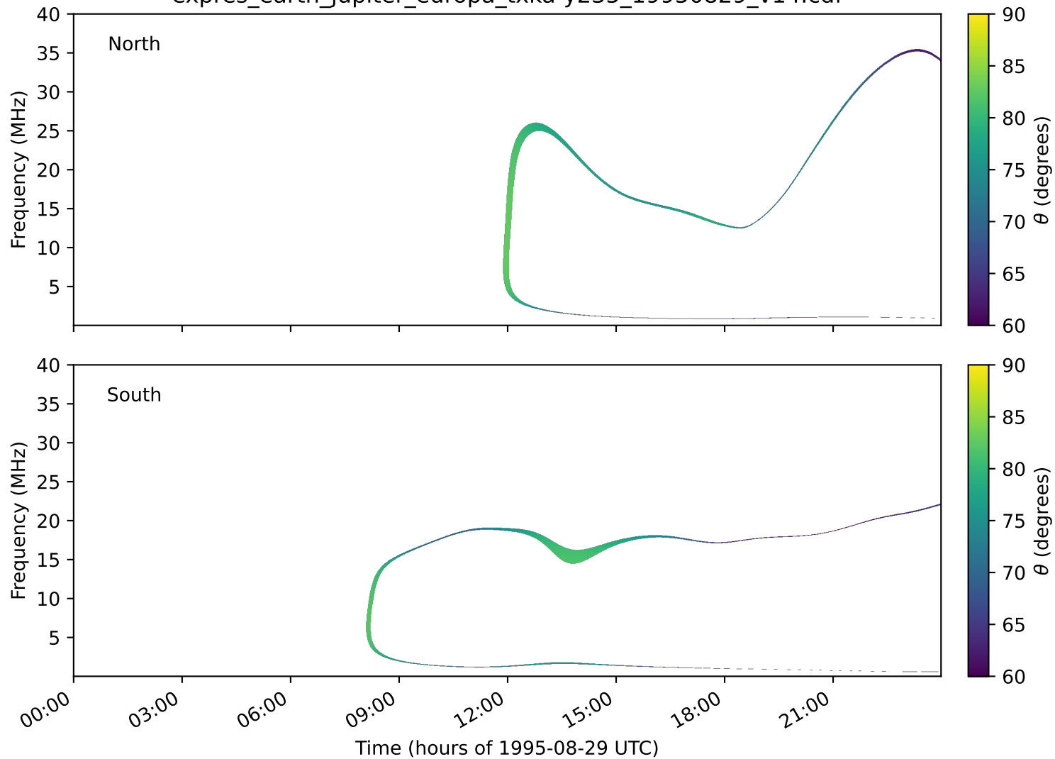
expres_earth_jupiter_europa_txka-y235_19950829_v14.cdf
