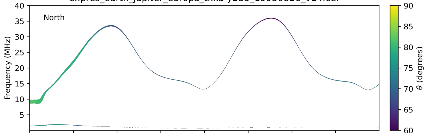
expres_earth_jupiter_europa_txka-y235_19950826_v14.cdf
