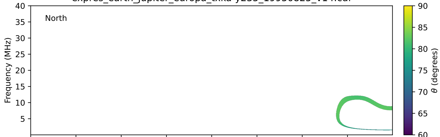
expres_earth_jupiter_europa_txka-y235_19950825_v14.cdf
