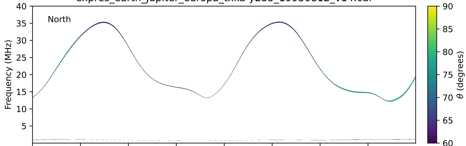
expres_earth_jupiter_europa_txka-y235_19950812_v14.cdf
