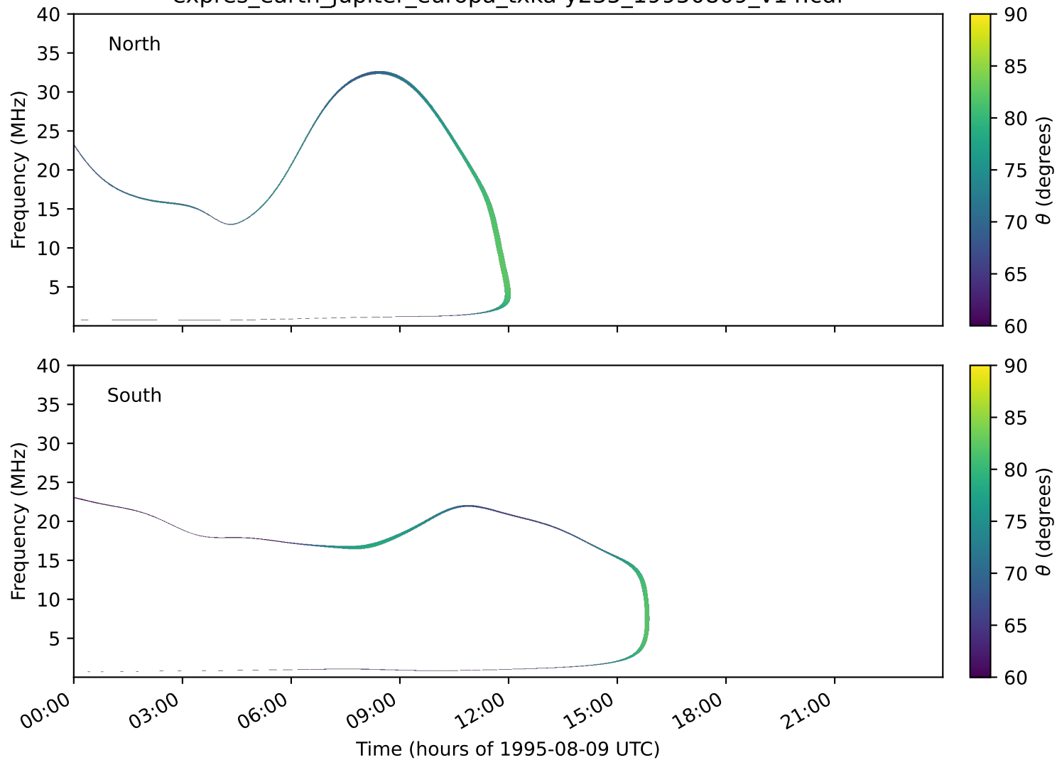
expres_earth_jupiter_europa_txka-y235_19950809_v14.cdf
