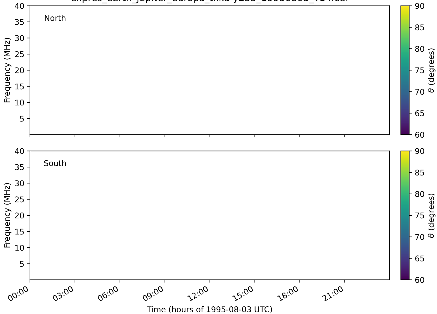
expres_earth_jupiter_europa_txka-y235_19950803_v14.cdf
