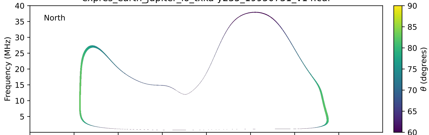
expres_earth_jupiter_io_txka-y235_19950731_v14.cdf
