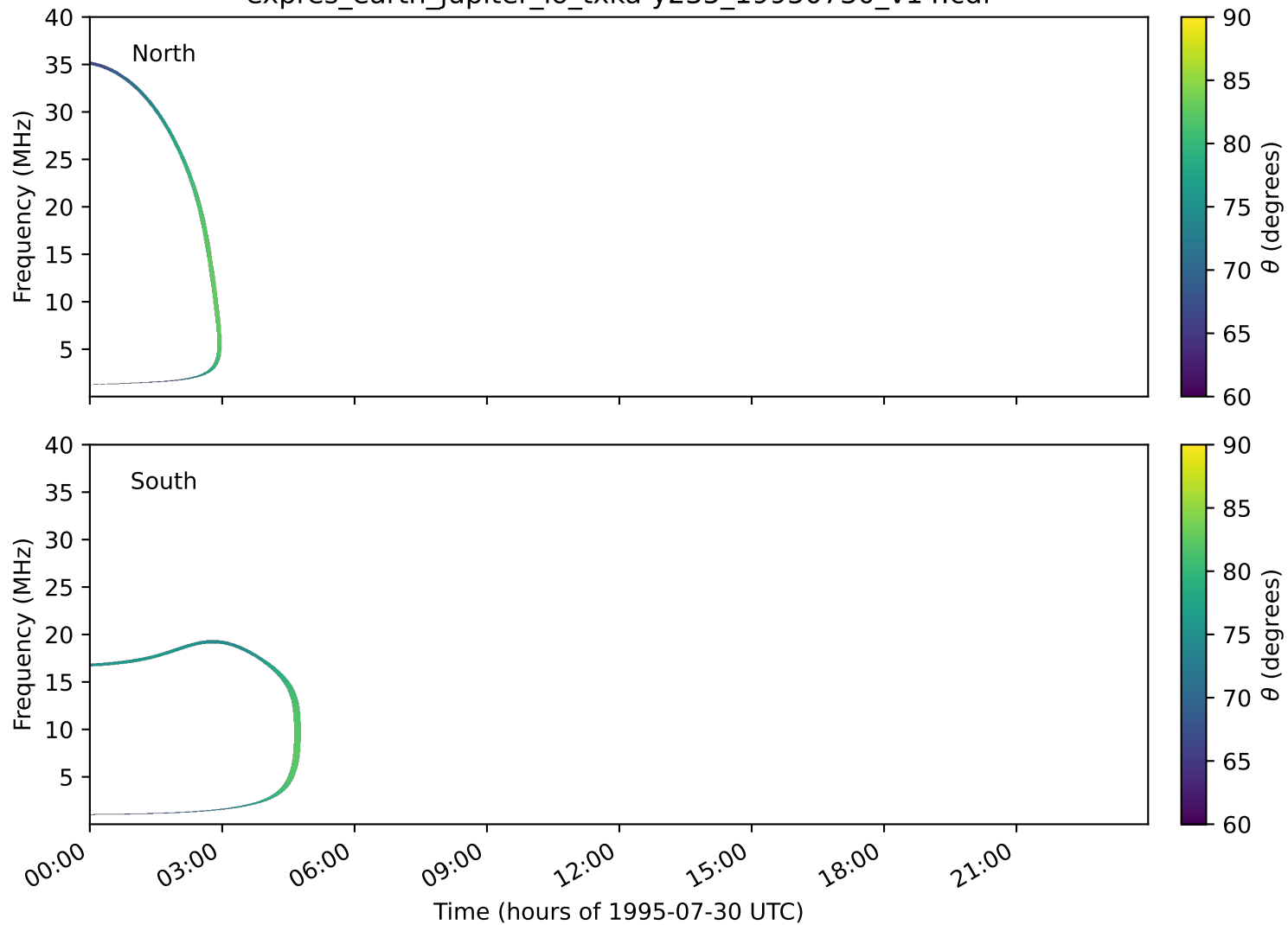
expres_earth_jupiter_io_txka-y235_19950730_v14.cdf
