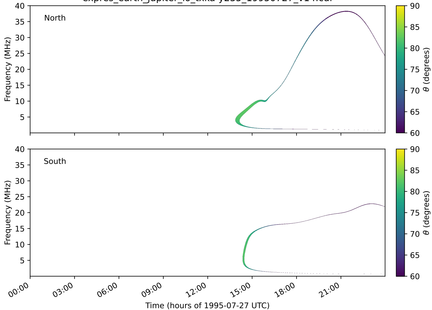
expres_earth_jupiter_io_txka-y235_19950727_v14.cdf
