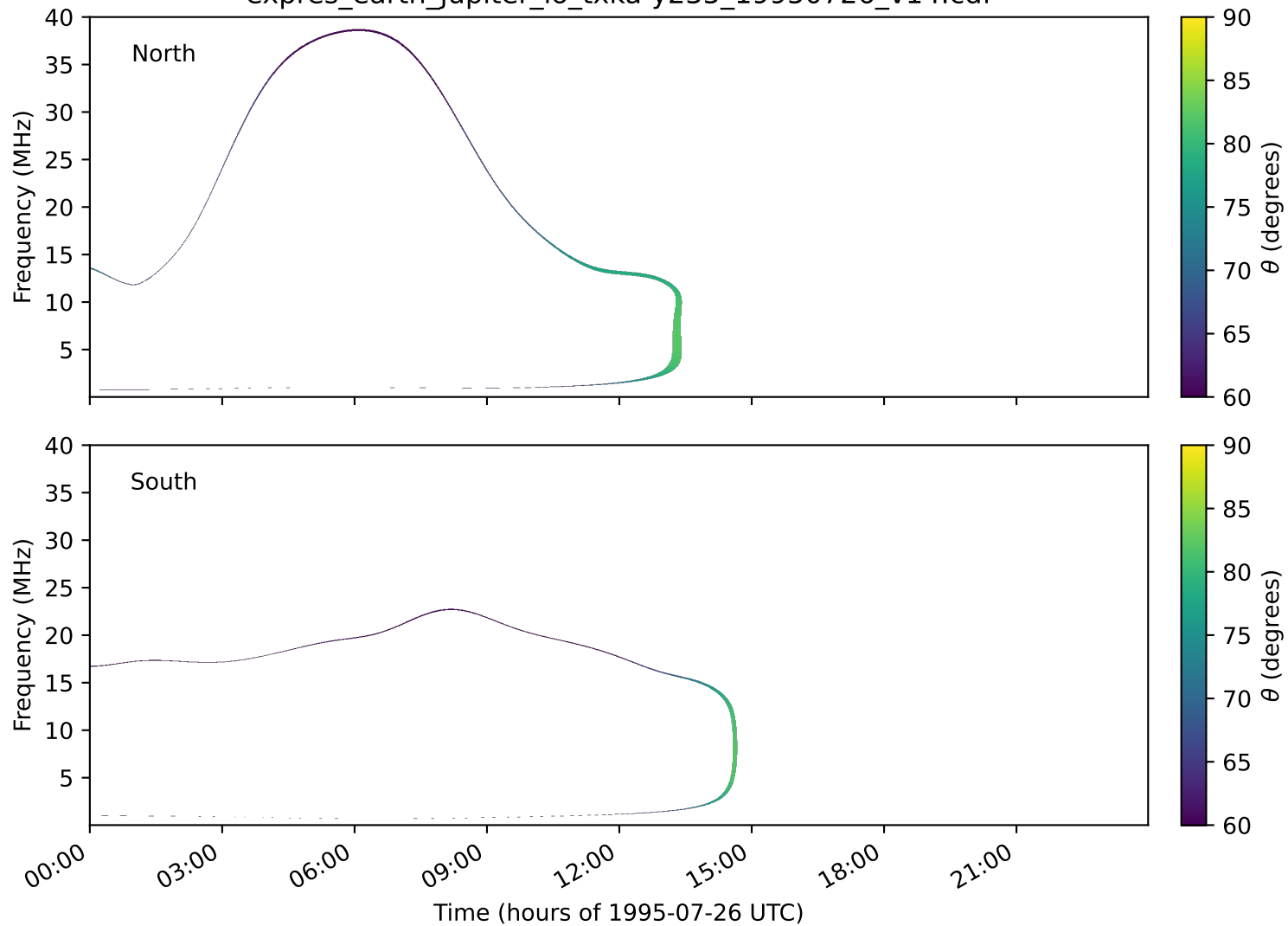
expres_earth_jupiter_io_txka-y235_19950726_v14.cdf
