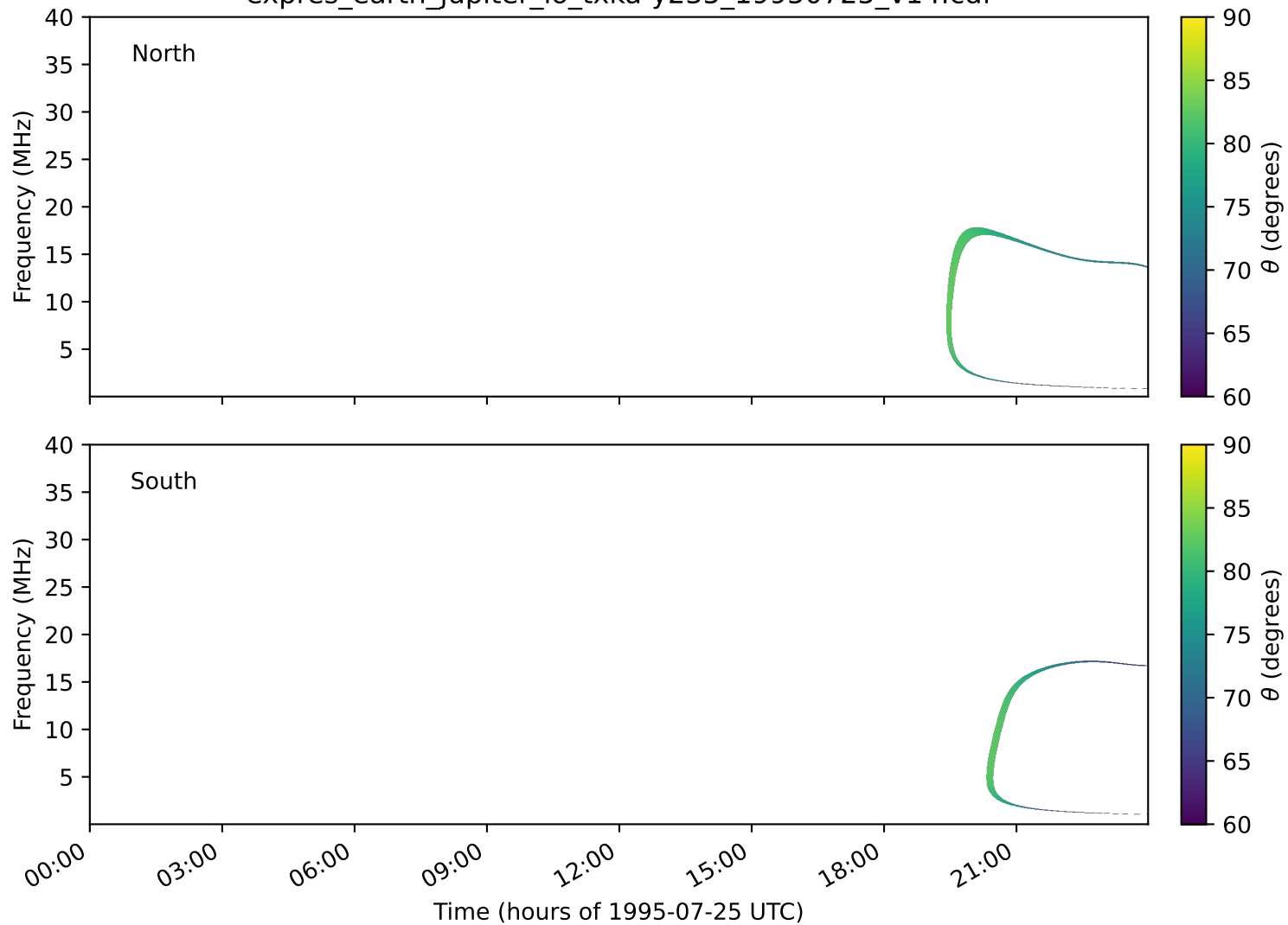
expres_earth_jupiter_io_txka-y235_19950725_v14.cdf
