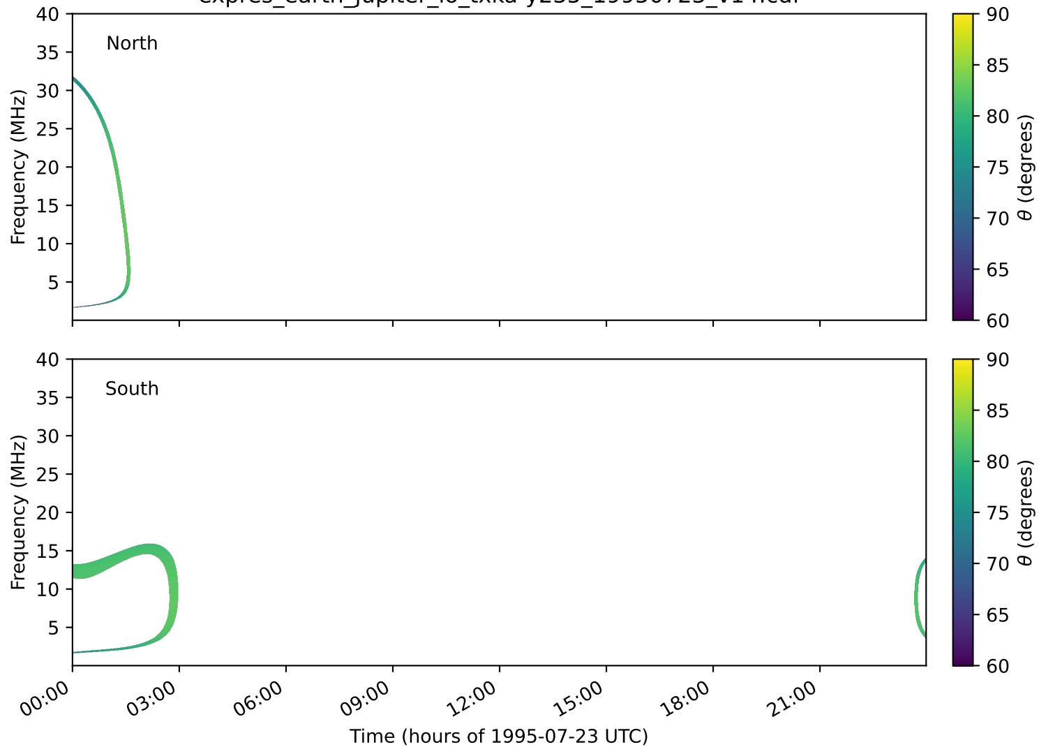
expres_earth_jupiter_io_txka-y235_19950723_v14.cdf
