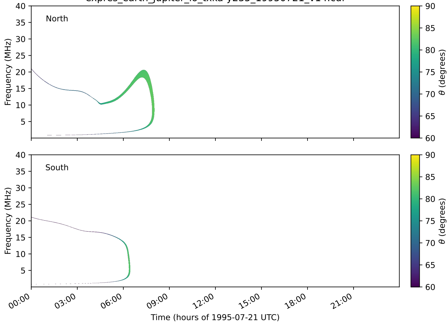
expres_earth_jupiter_io_txka-y235_19950721_v14.cdf
