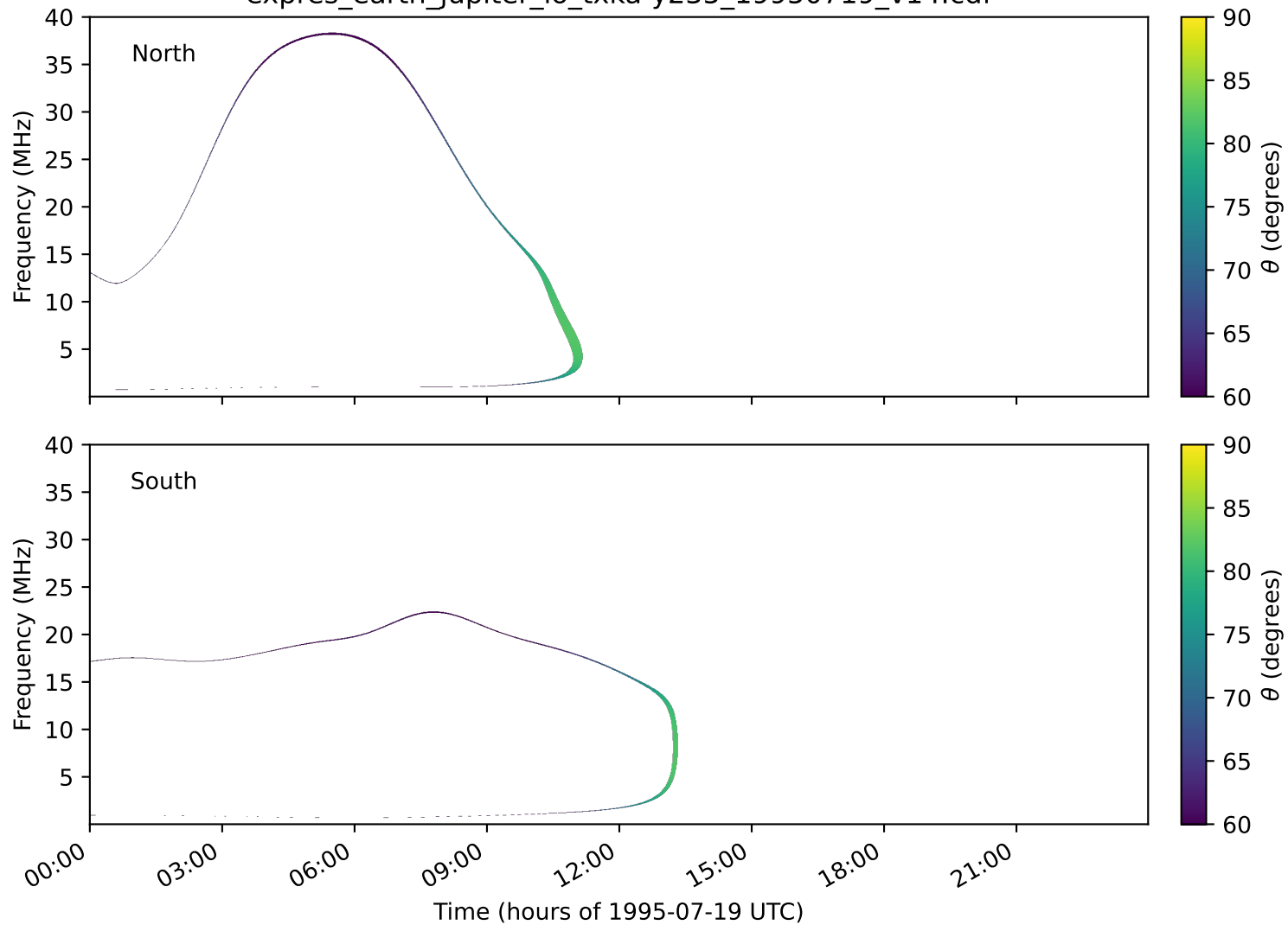
expres_earth_jupiter_io_txka-y235_19950719_v14.cdf
