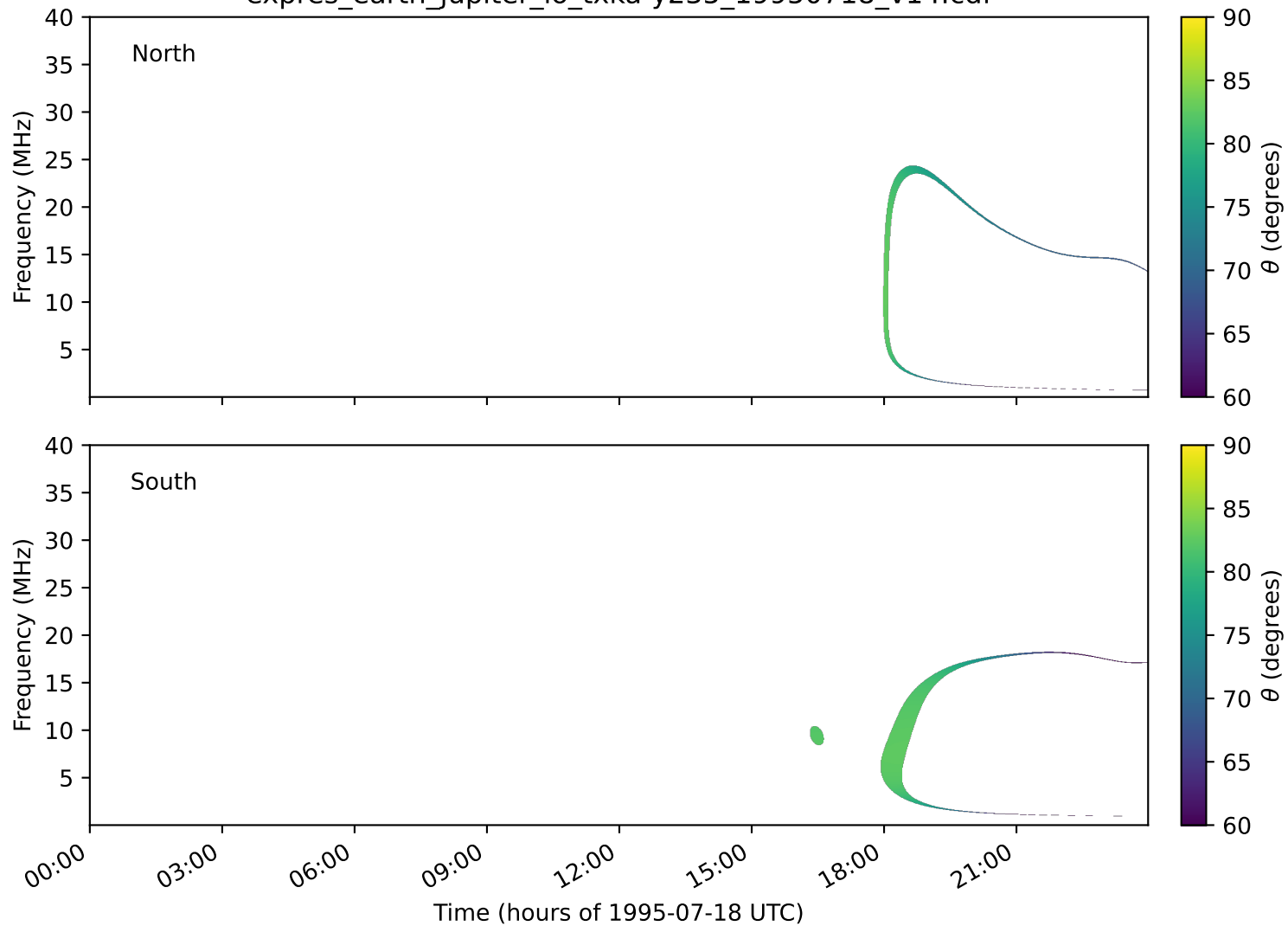
expres_earth_jupiter_io_txka-y235_19950718_v14.cdf
