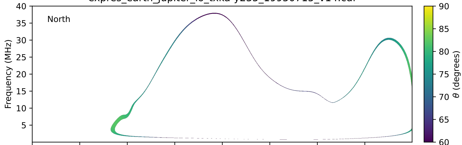
expres_earth_jupiter_io_txka-y235_19950715_v14.cdf
