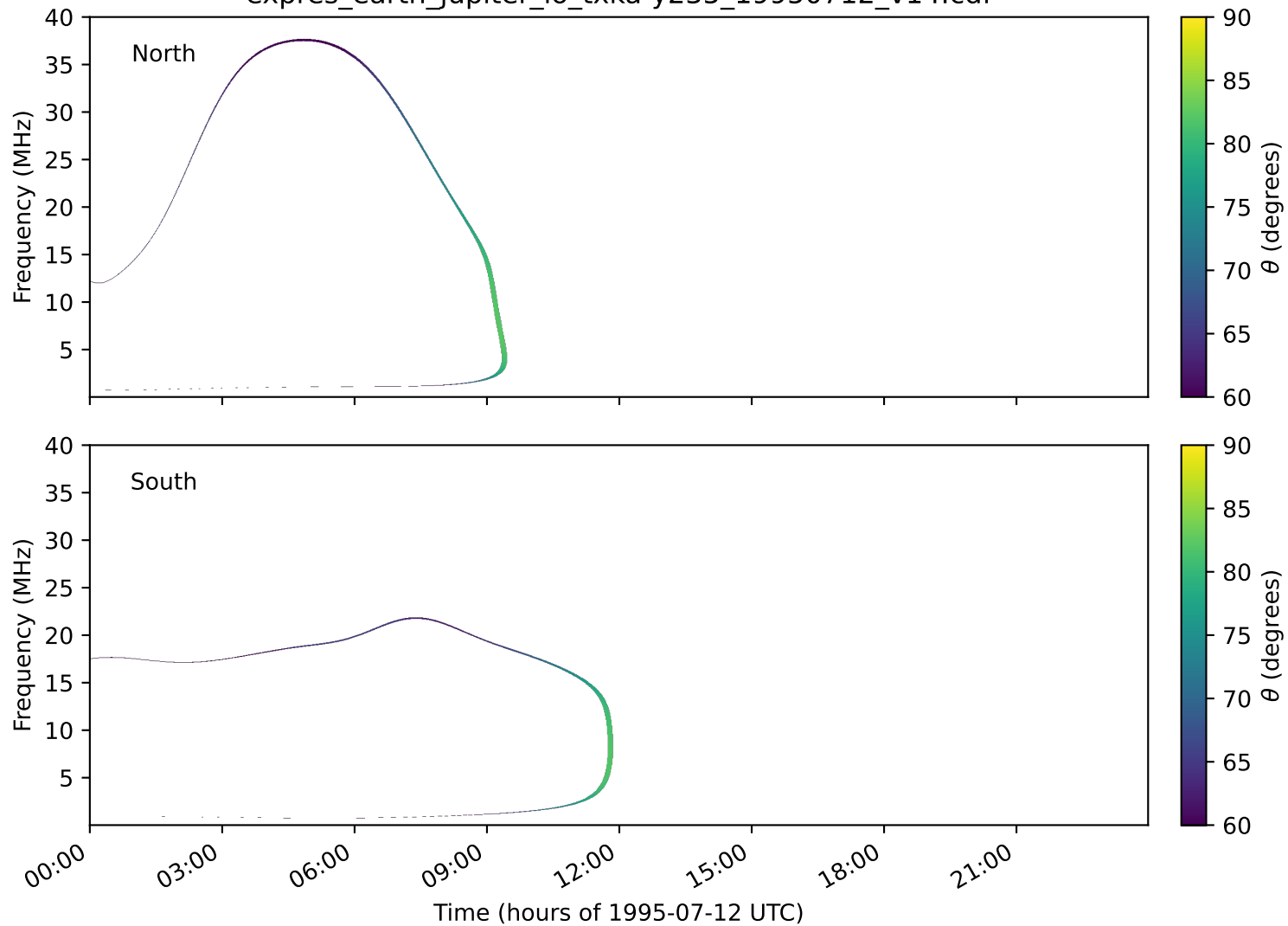
expres_earth_jupiter_io_txka-y235_19950712_v14.cdf
