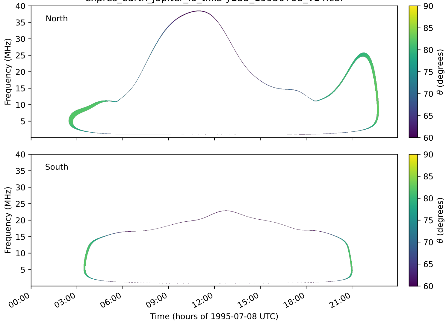
expres_earth_jupiter_io_txka-y235_19950708_v14.cdf
