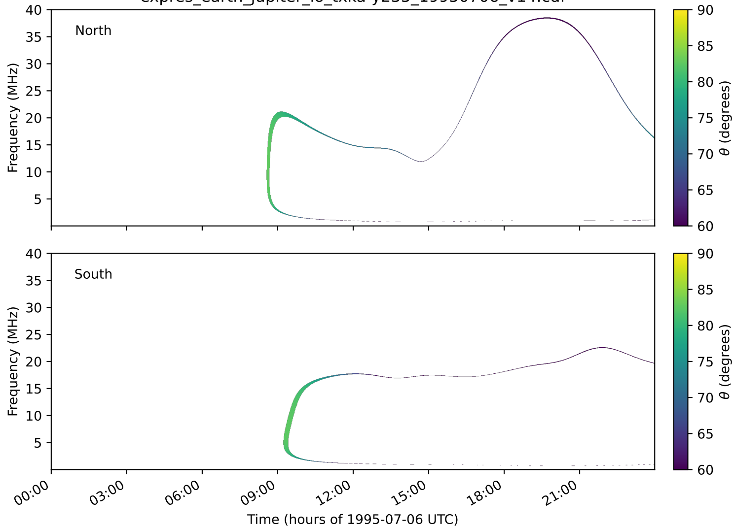
expres_earth_jupiter_io_txka-y235_19950706_v14.cdf
