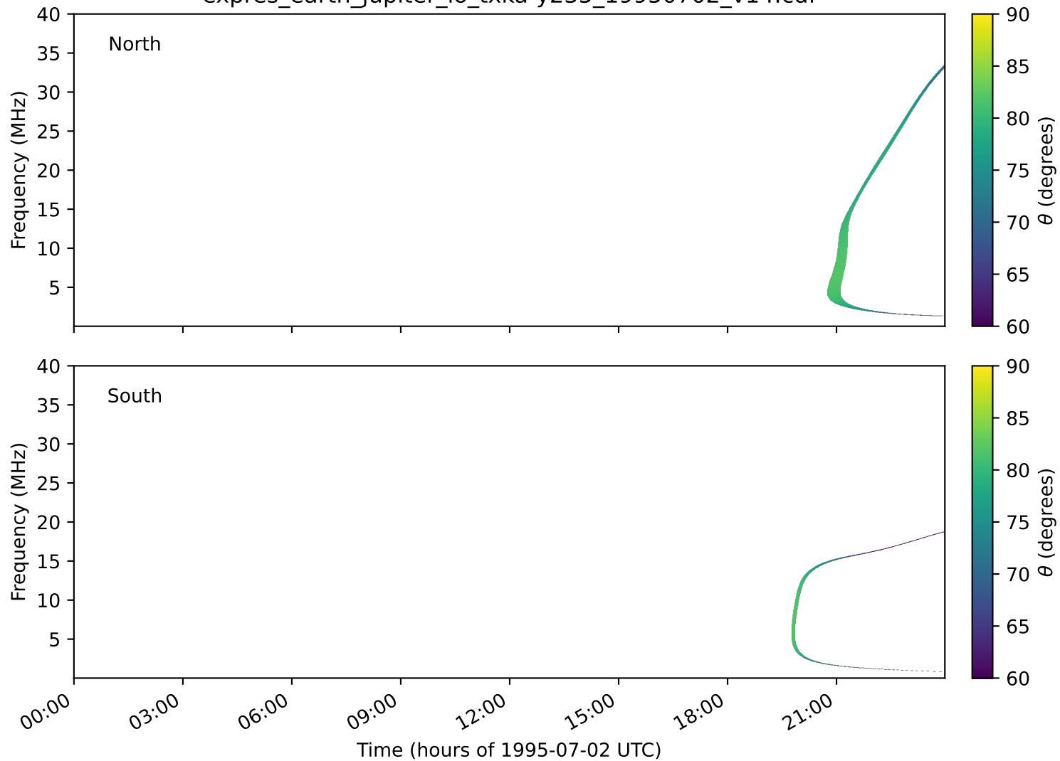
expres_earth_jupiter_io_txka-y235_19950702_v14.cdf
