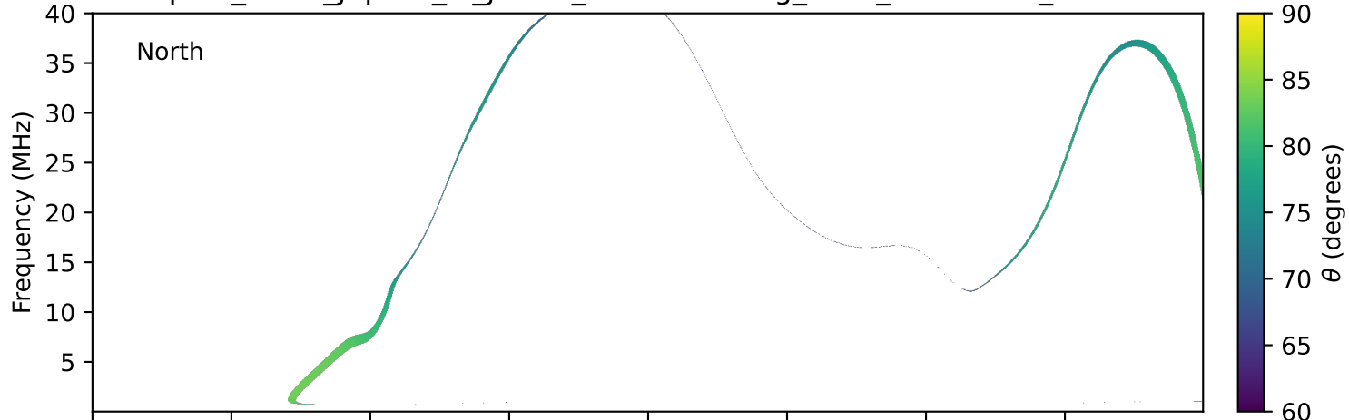
expres_earth_jupiter_io_jrm33_lossc-wid1deg_3kev_19950715_v11.cdf
