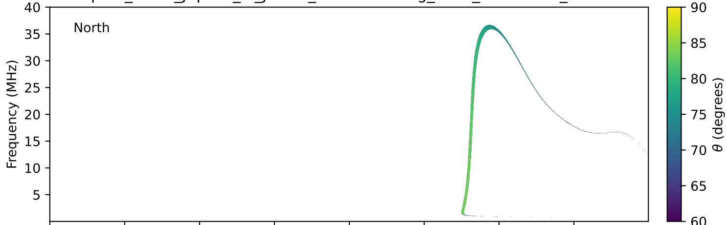
expres_earth_jupiter_io_jrm33_lossc-wid1deg_3kev_19950711_v11.cdf
