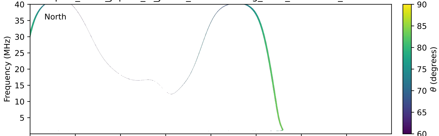
expres_earth_jupiter_io_jrm33_lossc-wid1deg_3kev_19950710_v11.cdf
