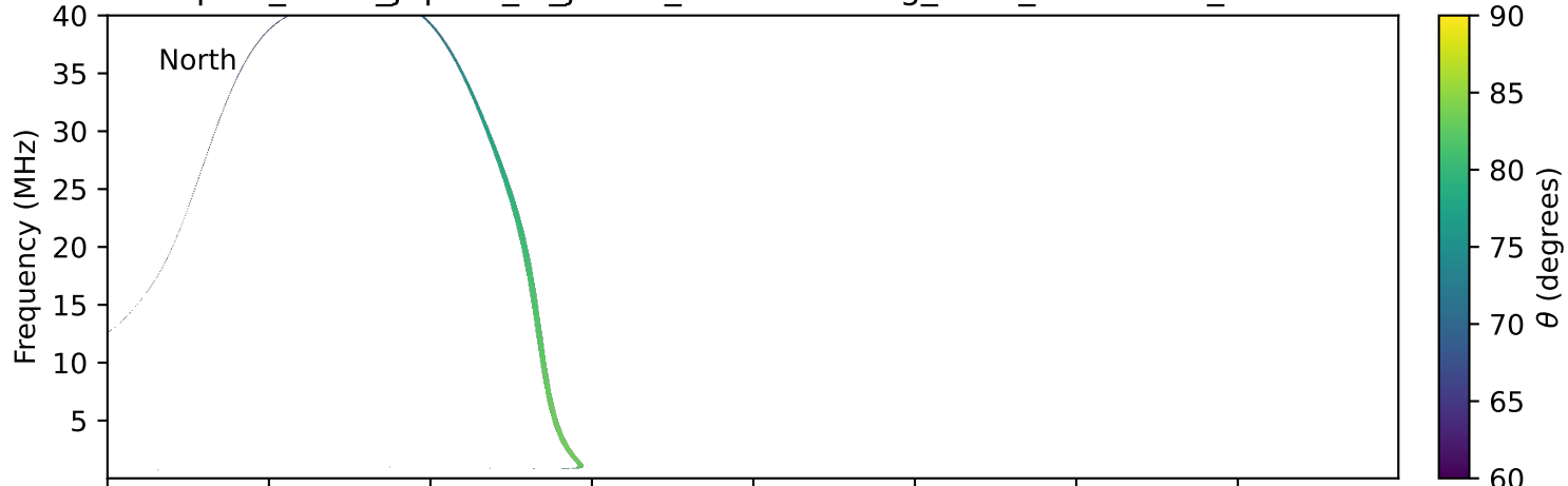
expres_earth_jupiter_io_jrm33_lossc-wid1deg_3kev_19950705_v11.cdf
