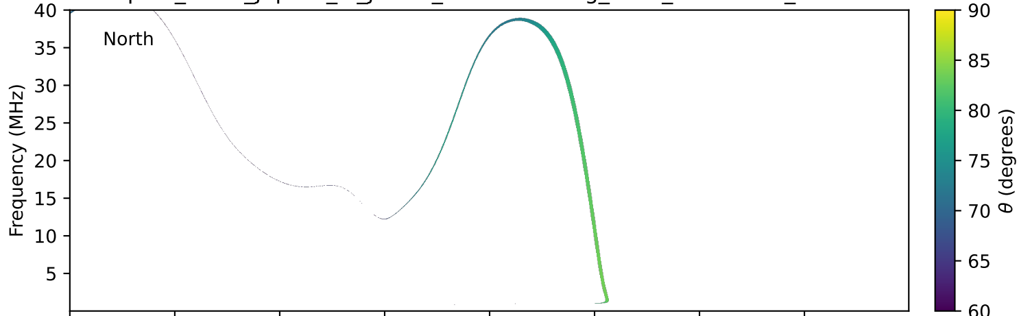
expres_earth_jupiter_io_jrm33_lossc-wid1deg_3kev_19950703_v11.cdf
