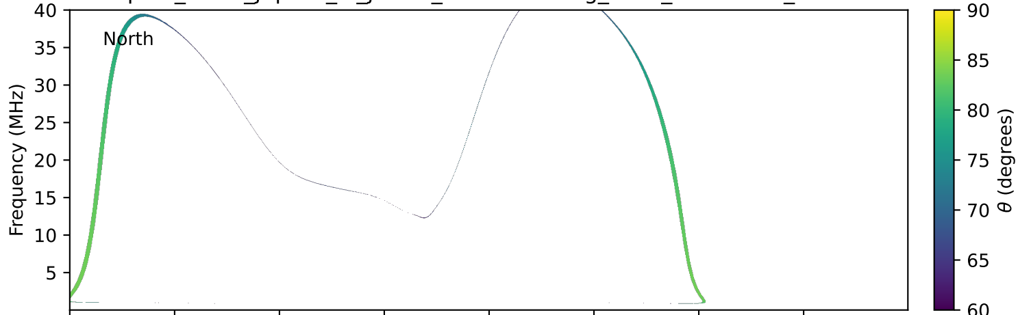
expres_earth_jupiter_io_jrm09_lossc-wid1deg_3kev_19950717_v11.cdf
