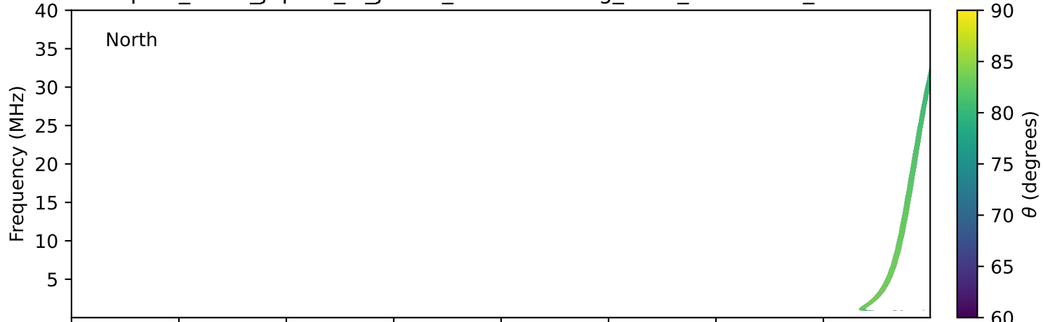
expres_earth_jupiter_io_jrm09_lossc-wid1deg_3kev_19950709_v11.cdf
